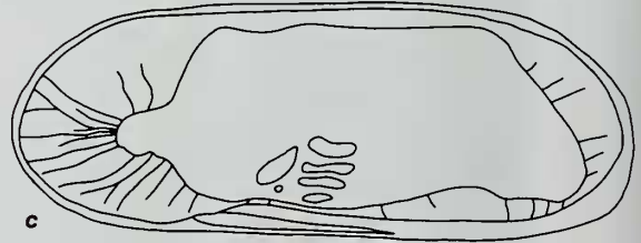
Fig. 7 Krithidae. Internal lateral views showing nature of marginal pore canals and muscle scar patterns. a, Krithe liebau sp. nov. Paratype, ♀ right valve OS 8161. \times 120 . b, Ommatokrithe prolata Ahmad. Holotype, ♀ left valve OS 7768. \times 100 . c, Parakrithe cicatricosa sp. nov. Paratype, ♀ right valve OS 8169. \times 150 .
